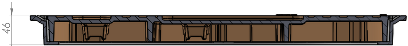
SECTION A-A SCALE 1 : 3.5
